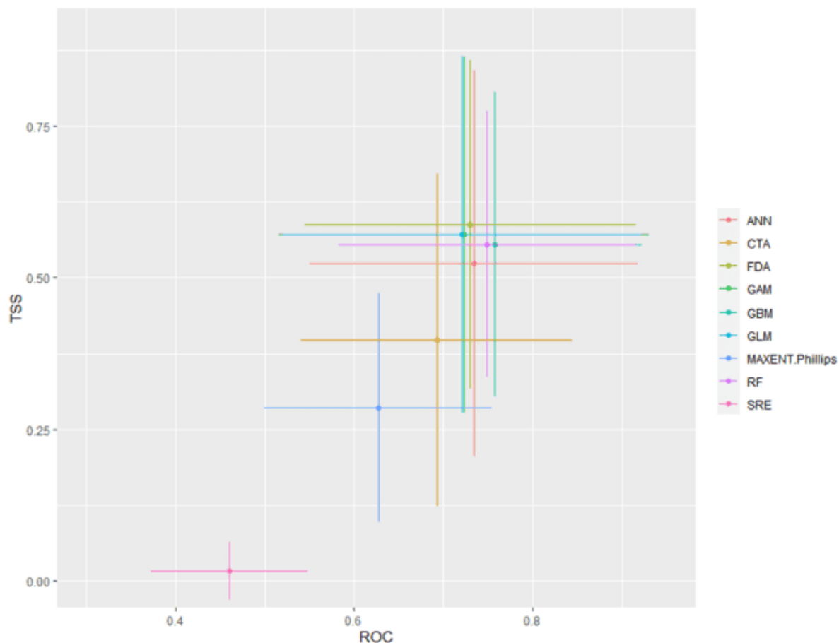
Figure 3. Presents a scatter plot comparing different statistical models based on two metrics: Receiver Operating Characteristic (ROC) and True Skill Statistics (TSS). Each point on the plot represents a model's performance, with the horizontal axis showing the ROC value and the vertical axis showing the TSS value. The inclusion of error bars indicates variability or uncertainty in the measurements, which suggests that the model performance can vary under different conditions or datasets. Models such as Random Forest (RF) and Generalized Linear Models (GLM) show differing levels of performance based on these metrics.
